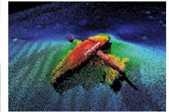
GeoSwath MBES image of target.
